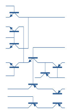
S11 (5 x NPN + 6 x PNP)
