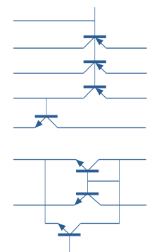
S17 (4 x NPN + 3 x PNP)
