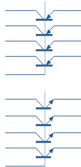
S2 (4 x NPN + 4 x PNP)
